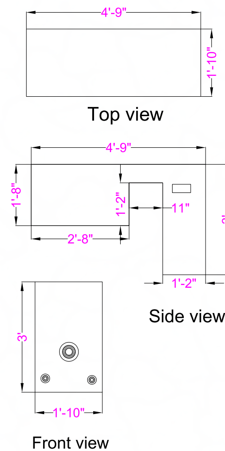
RETROFIT PIPELESS FILTER
