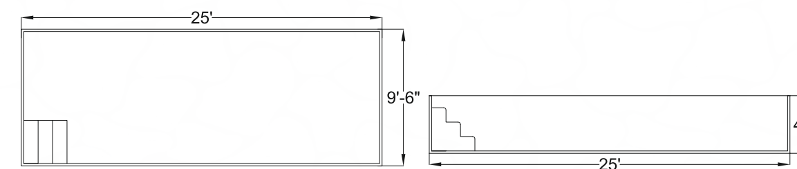
RECTANGULAR SWIMMING POOL - (25'X9.6'X4') MODEL - W3
